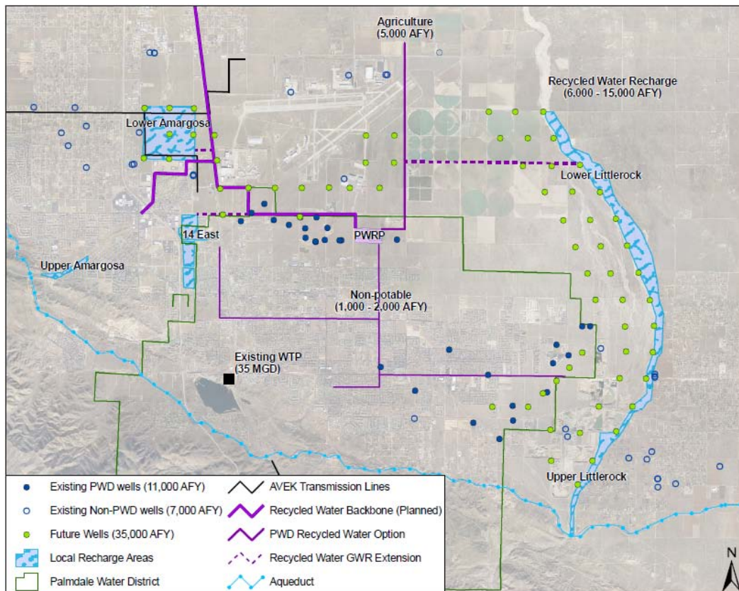
Figure 3-2: Proposed Well and Groundwater Recharge Siting
